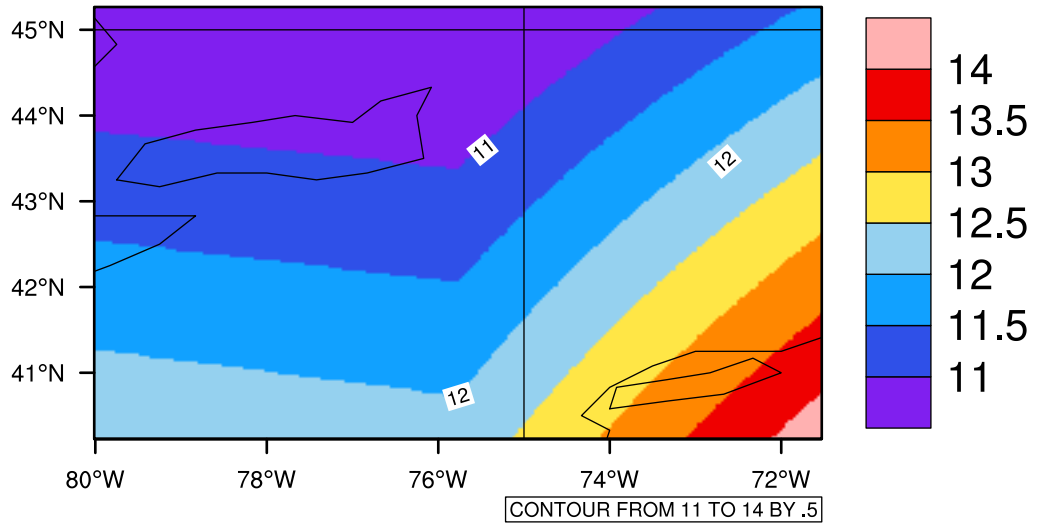
Yearly tasmax(c) In 2060-2069 GFDL-ESM2M RCP45 - New York
