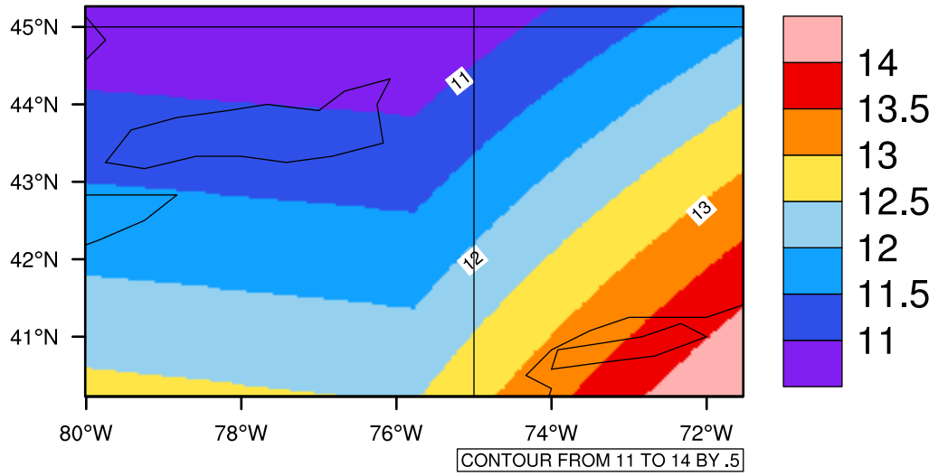
Yearly tasmax(c) In 2070-2079 GFDL-ESM2M RCP45 - New York
