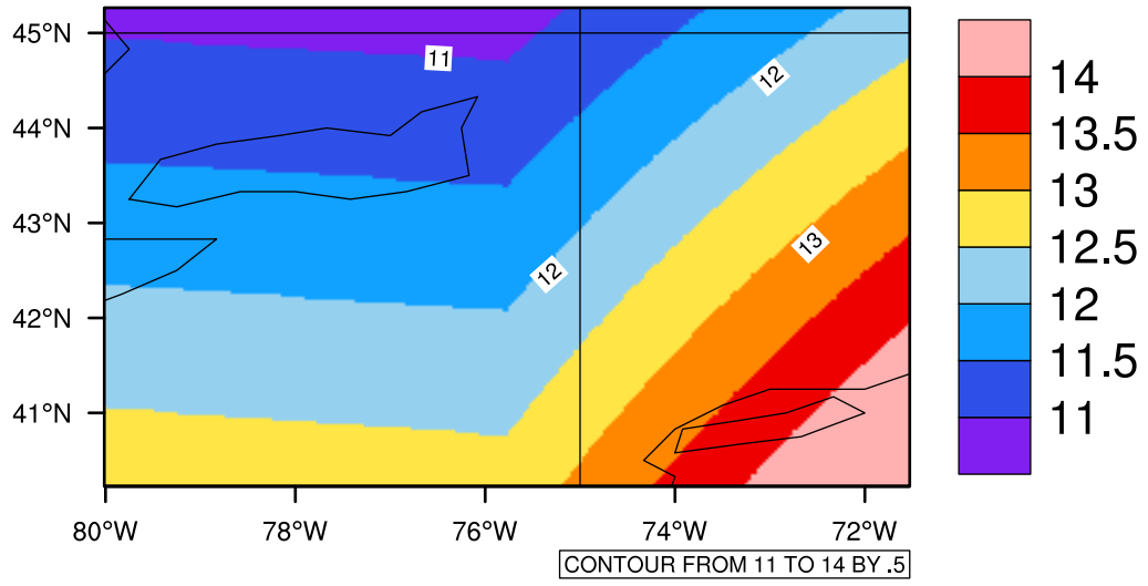
Yearly tasmax(c) In 2080-2089 GFDL-ESM2M RCP45 - New York
