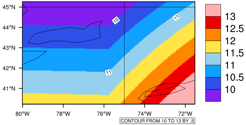
Yearly tasmax(c) In 2020-2029 GFDL-ESM2M RCP85 - New York
