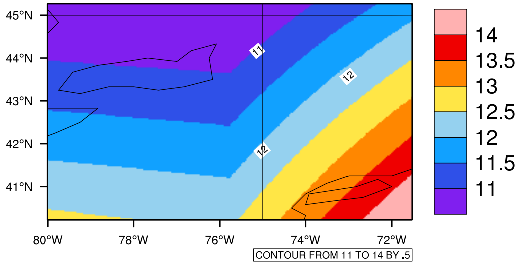
Yearly tasmax(c) In 2030-2039 GFDL-ESM2M RCP85 - New York
