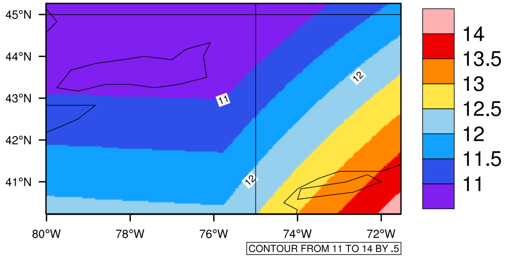
Yearly tasmax(c) In 2040-2049 GFDL-ESM2M RCP85 - New York
