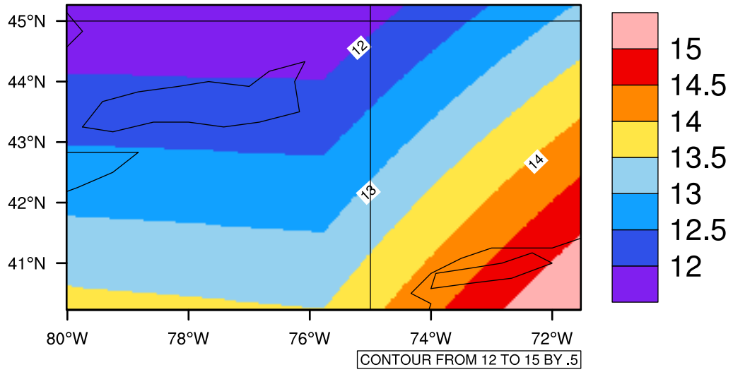
Yearly tasmax(c) In 2050-2059 GFDL-ESM2M RCP85 - New York
