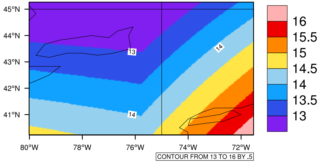
Yearly tasmax(c) In 2070-2079 GFDL-ESM2M RCP85 - New York
