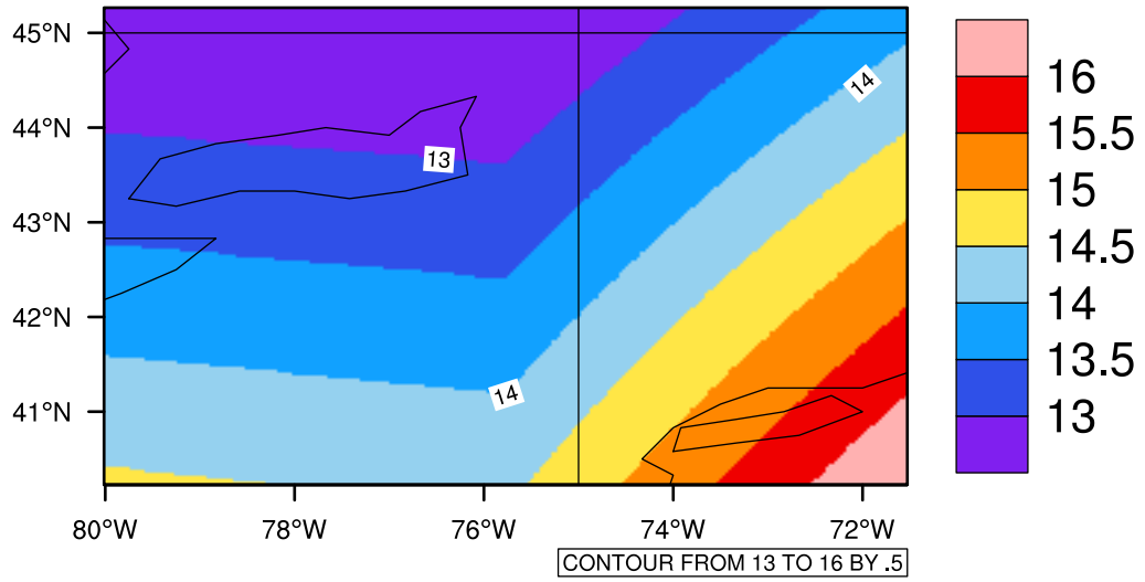
Yearly tasmax(c) In 2080-2089 GFDL-ESM2M RCP85 - New York
