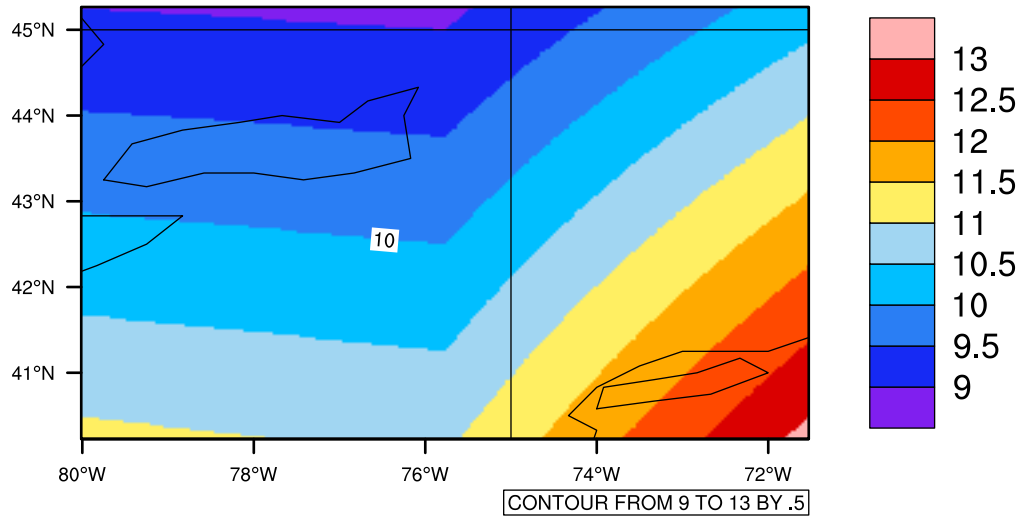
Yearly tasmax(c) In 1975-2005 GFDL-ESM2M historical - New York
