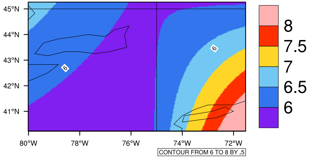
Yearly tasmin(c) In 2060-2069 GFDL-ESM2M RCP45 - New York
