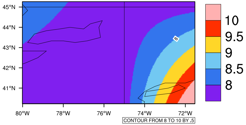
Yearly tasmin(c) In 2070-2079 GFDL-ESM2M RCP85 - New York
