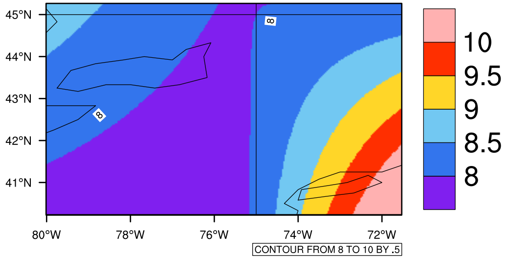
Yearly tasmin(c) In 2080-2089 GFDL-ESM2M RCP85 - New York
