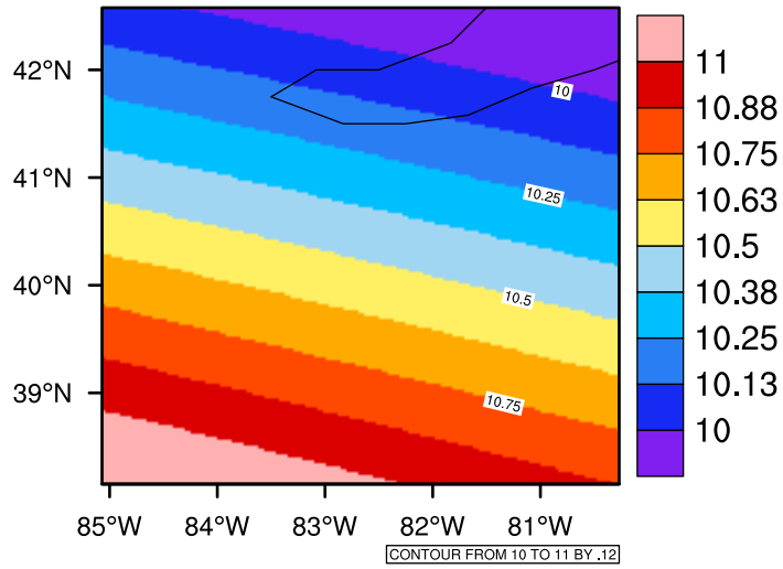
Yearly tas(c) In 2060-2069 GFDL-ESM2M RCP45 - Ohio
