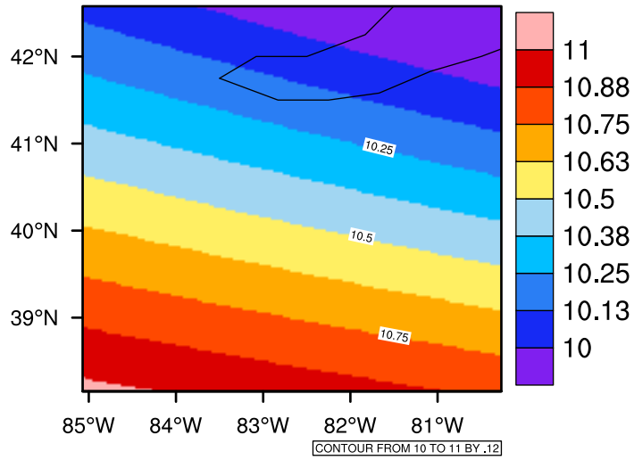
Yearly tas(c) In 2030-2039 GFDL-ESM2M RCP85 - Ohio
