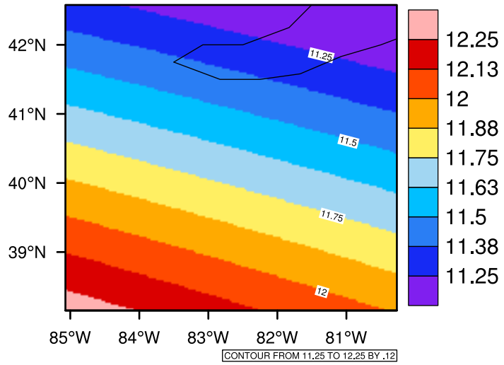
Yearly tas(c) In 2060-2069 GFDL-ESM2M RCP85 - Ohio
