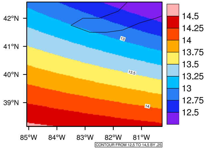
Yearly tasmax(c) In 2040-2049 GFDL-ESM2M RCP85 - Ohio
