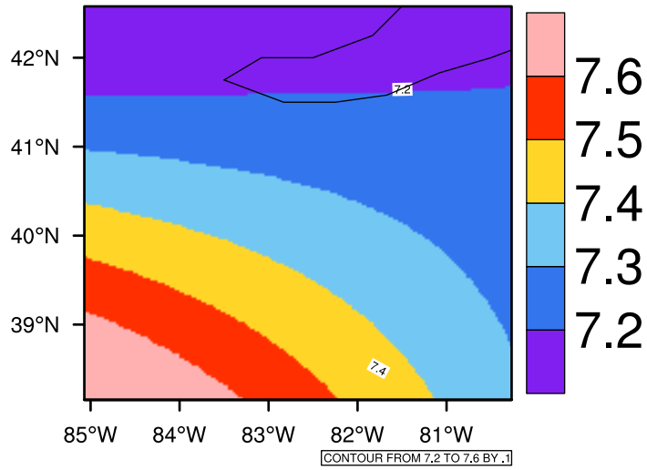
Yearly tasmin(c) In 2030-2039 GFDL-ESM2M RCP45 - Ohio
