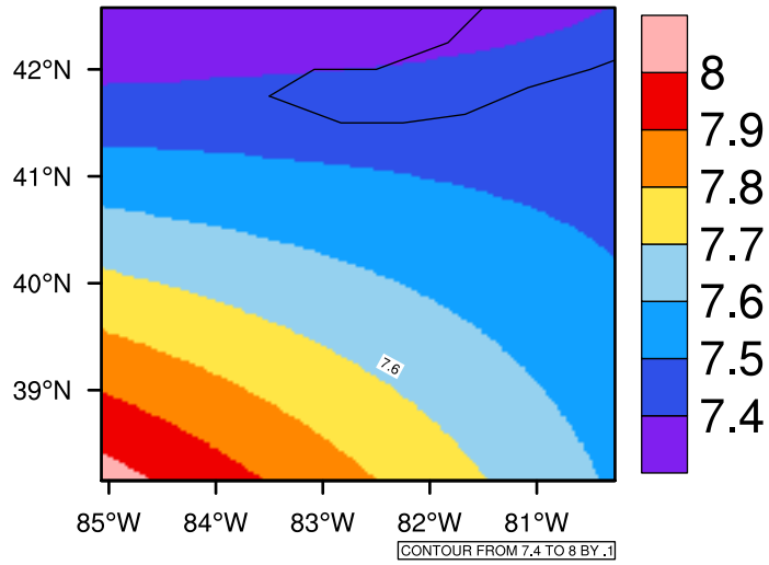
Yearly tasmin(c) In 2040-2049 GFDL-ESM2M RCP45 - Ohio
