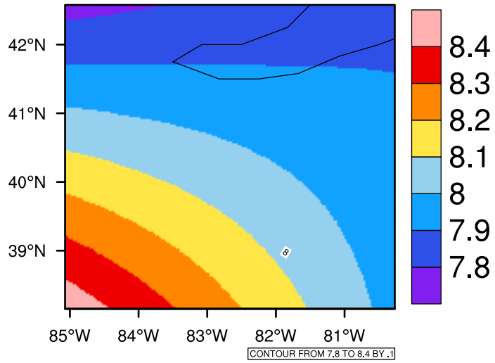
Yearly tasmin(c) In 2080-2089 GFDL-ESM2M RCP45 - Ohio
