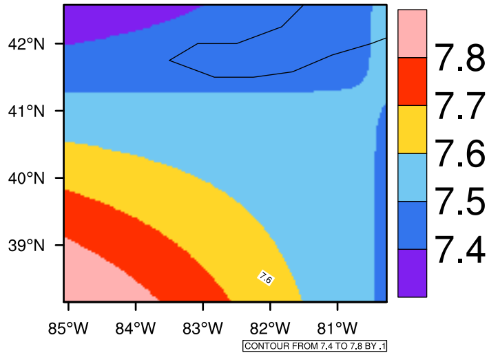
Yearly tasmin(c) In 2090-2099 GFDL-ESM2M RCP45 - Ohio
