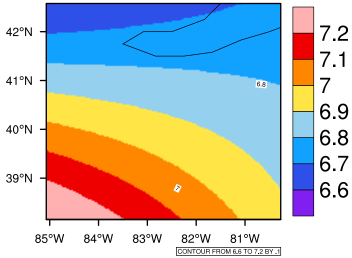
Yearly tasmin(c) In 2020-2029 GFDL-ESM2M RCP85 - Ohio
