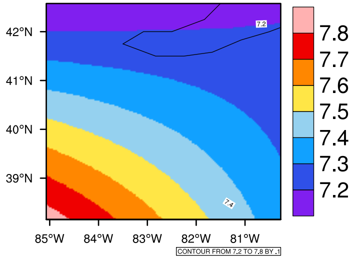
Yearly tasmin(c) In 2040-2049 GFDL-ESM2M RCP85 - Ohio
