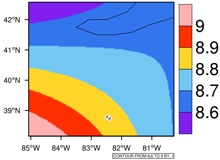
Yearly tasmin(c) In 2060-2069 GFDL-ESM2M RCP85 - Ohio
