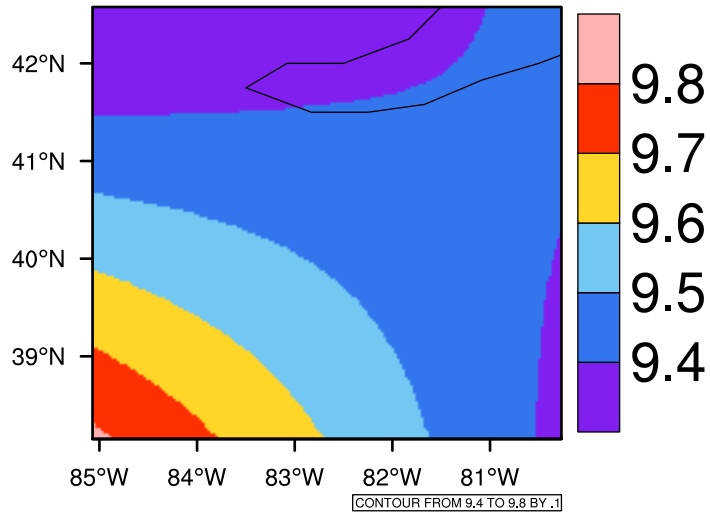
Yearly tasmin(c) In 2080-2089 GFDL-ESM2M RCP85 - Ohio
