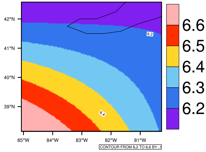
Yearly tasmin(c) In 1975-2005 GFDL-ESM2M historical - Ohio
