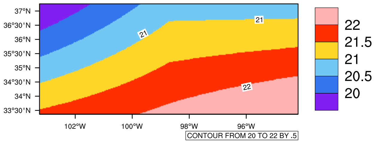
Yearly tasmax(c) In 2030-2039 GFDL-ESM2M RCP45 - Oklahoma
