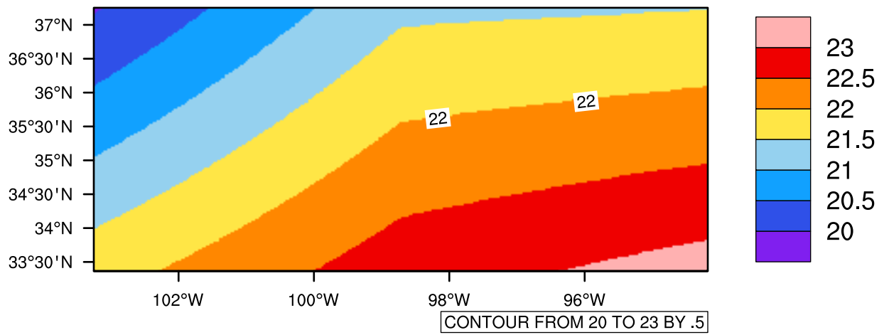
Yearly tasmax(c) In 2070-2079 GFDL-ESM2M RCP45 - Oklahoma
