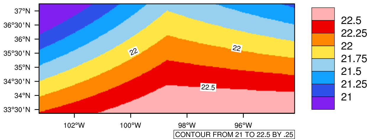
Yearly tasmax(c) In 2090-2099 GFDL-ESM2M RCP45 - Oklahoma
