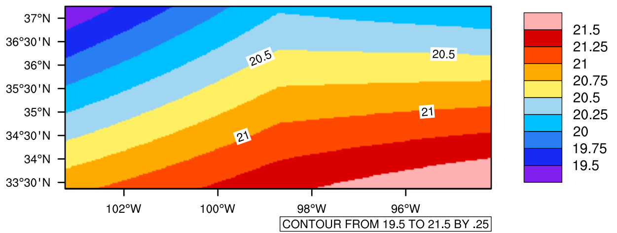
Yearly tasmax(c) In 2020-2029 GFDL-ESM2M RCP85 - Oklahoma
