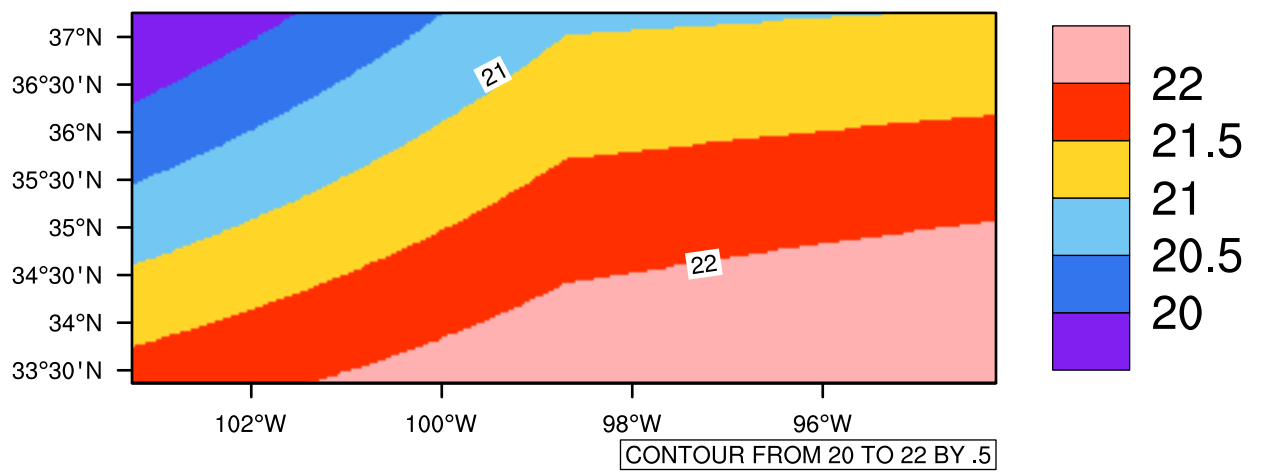
Yearly tasmax(c) In 2030-2039 GFDL-ESM2M RCP85 - Oklahoma
