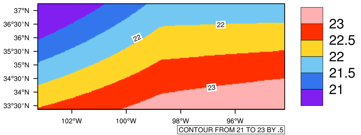
Yearly tasmax(c) In 2050-2059 GFDL-ESM2M RCP85 - Oklahoma
