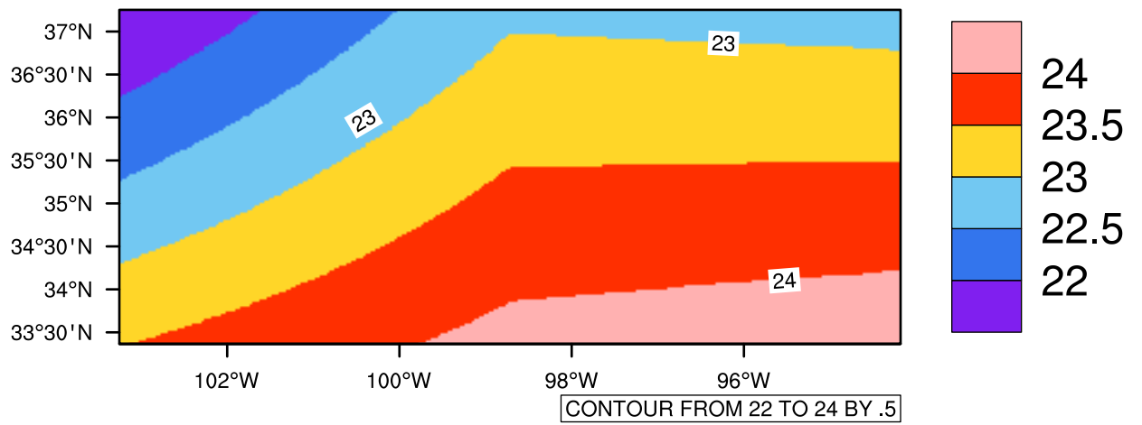
Yearly tasmax(c) In 2060-2069 GFDL-ESM2M RCP85 - Oklahoma
