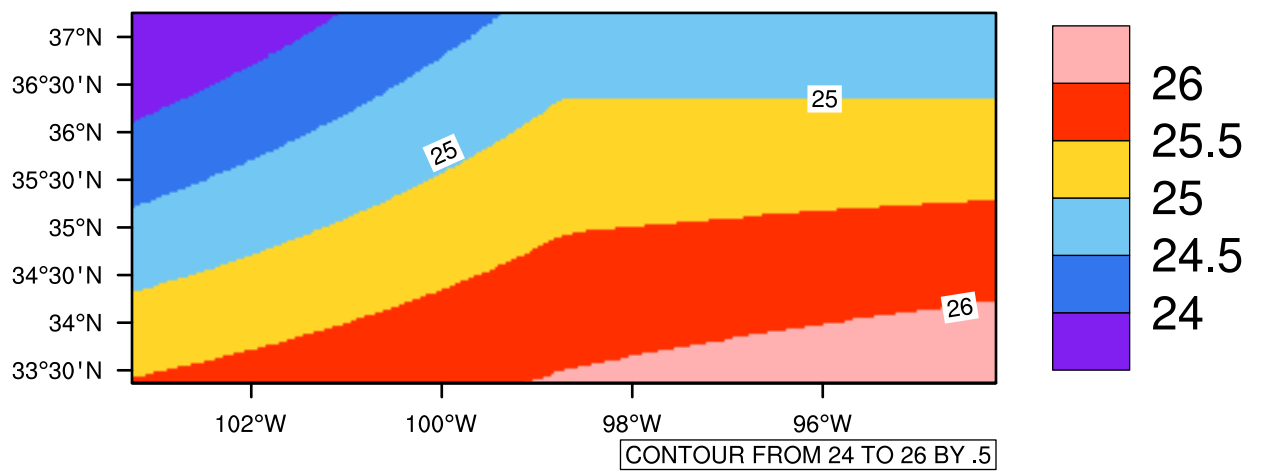
Yearly tasmax(c) In 2090-2099 GFDL-ESM2M RCP85 - Oklahoma
