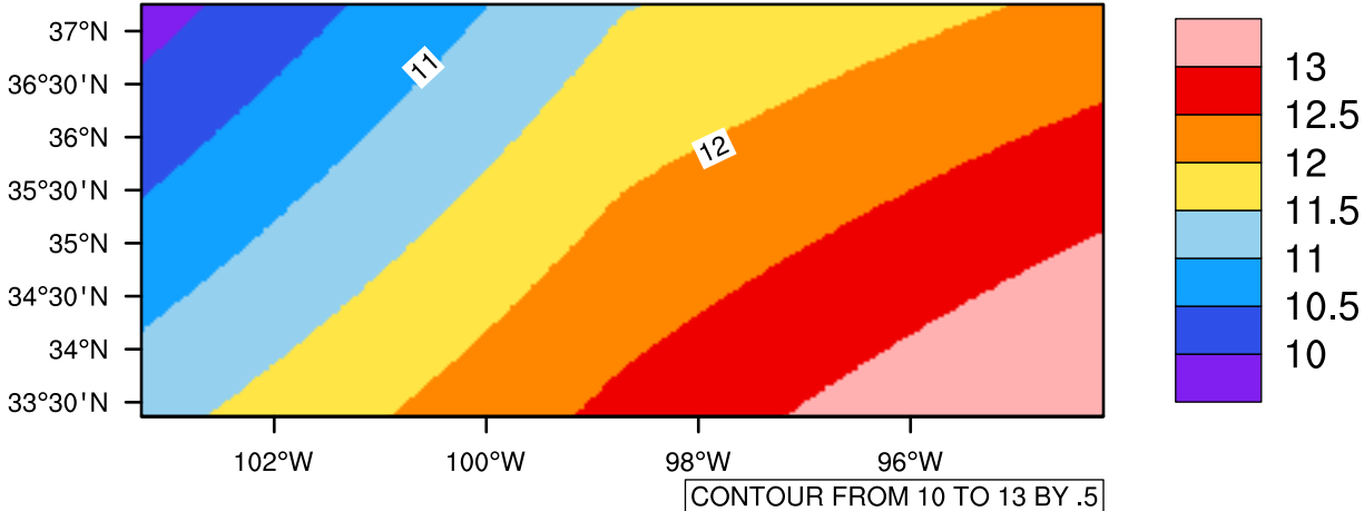
Yearly tasmin(c) In 2040-2049 GFDL-ESM2M RCP45 - Oklahoma
