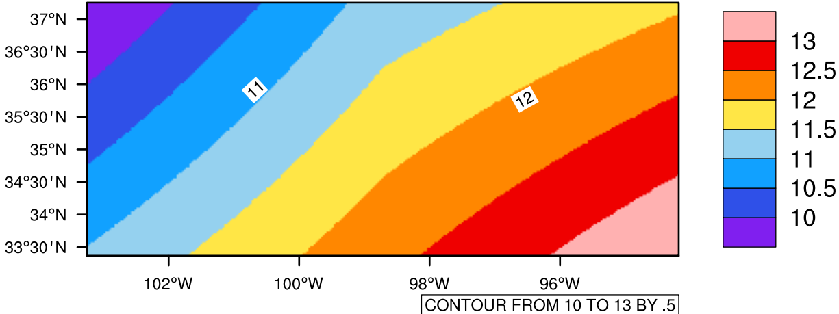
Yearly tasmin(c) In 2060-2069 GFDL-ESM2M RCP45 - Oklahoma
