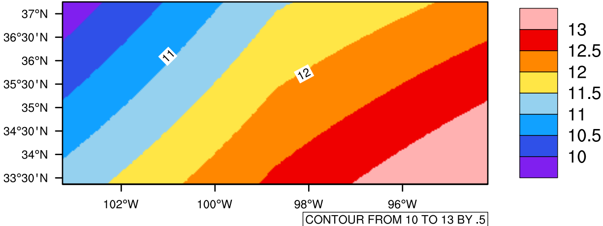
Yearly tasmin(c) In 2070-2079 GFDL-ESM2M RCP45 - Oklahoma
