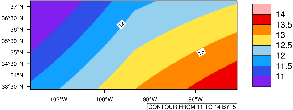
Yearly tasmin(c) In 2080-2089 GFDL-ESM2M RCP45 - Oklahoma
