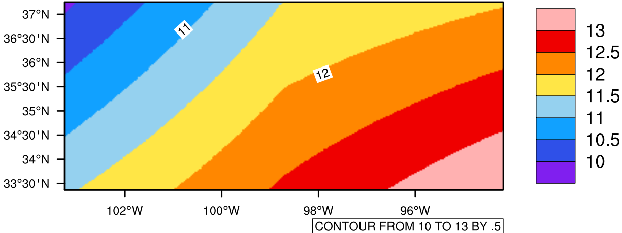
Yearly tasmin(c) In 2090-2099 GFDL-ESM2M RCP45 - Oklahoma
