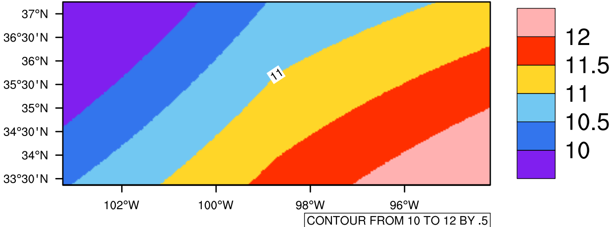
Yearly tasmin(c) In 2020-2029 GFDL-ESM2M RCP85 - Oklahoma
