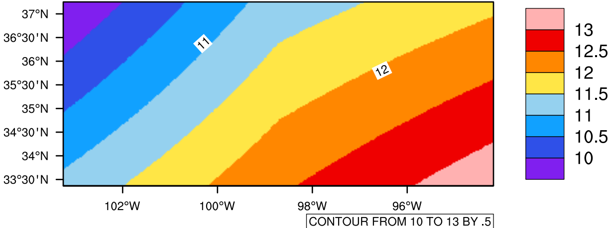
Yearly tasmin(c) In 2040-2049 GFDL-ESM2M RCP85 - Oklahoma
