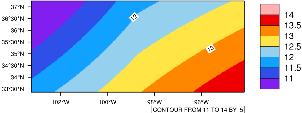
Yearly tasmin(c) In 2050-2059 GFDL-ESM2M RCP85 - Oklahoma
