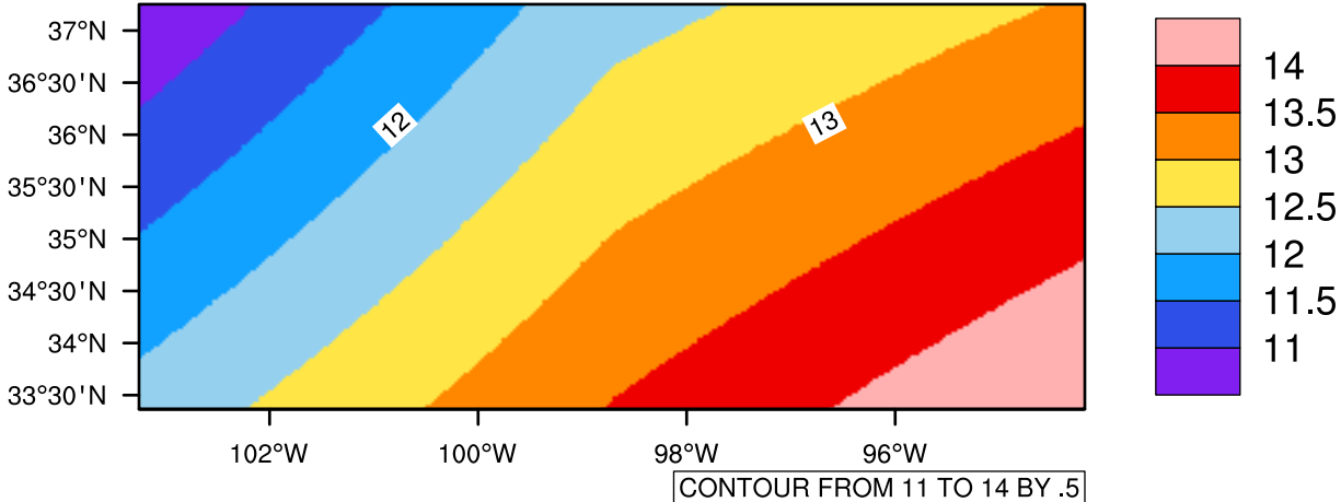
Yearly tasmin(c) In 2060-2069 GFDL-ESM2M RCP85 - Oklahoma
