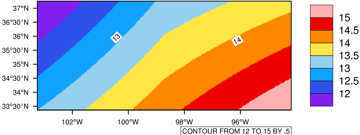
Yearly tasmin(c) In 2080-2089 GFDL-ESM2M RCP85 - Oklahoma
