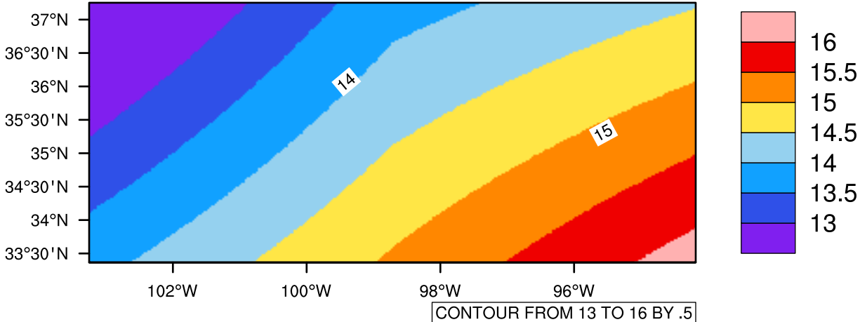
Yearly tasmin(c) In 2090-2099 GFDL-ESM2M RCP85 - Oklahoma
