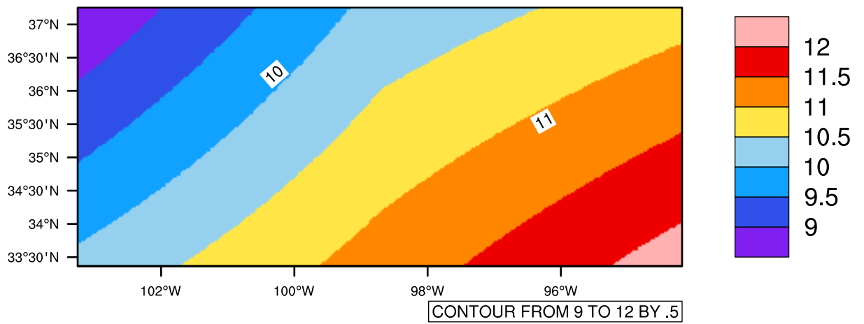
Yearly tasmin(c) In 1975-2005 GFDL-ESM2M historical - Oklahoma
