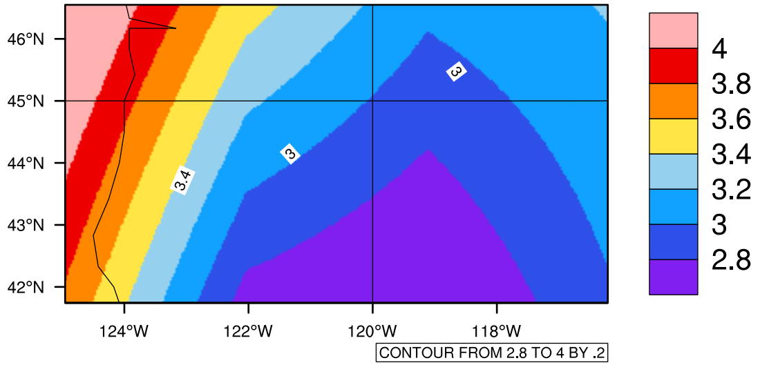
Yearly pr (mm/day) In 2040-2049 GFDL-ESM2M RCP45 - Oregon
