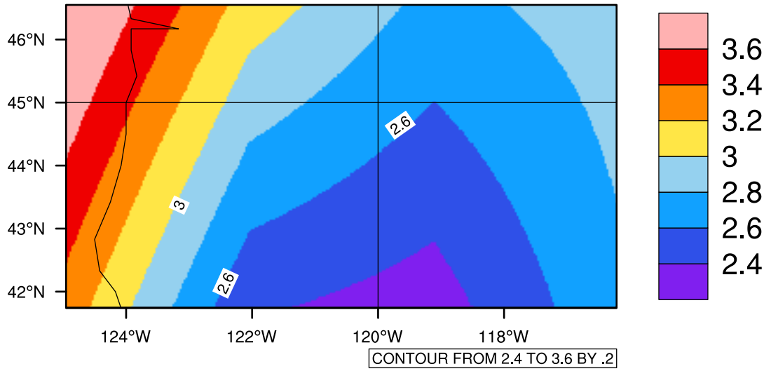
Yearly pr (mm/day) In 2060-2069 GFDL-ESM2M RCP45 - Oregon
