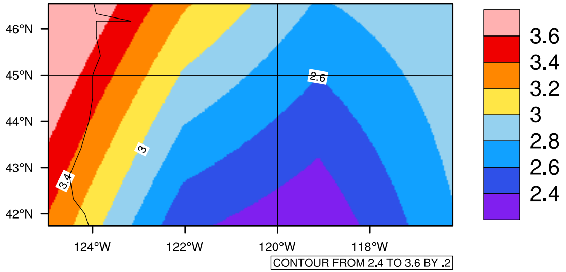
Yearly pr (mm/day) In 2070-2079 GFDL-ESM2M RCP45 - Oregon
