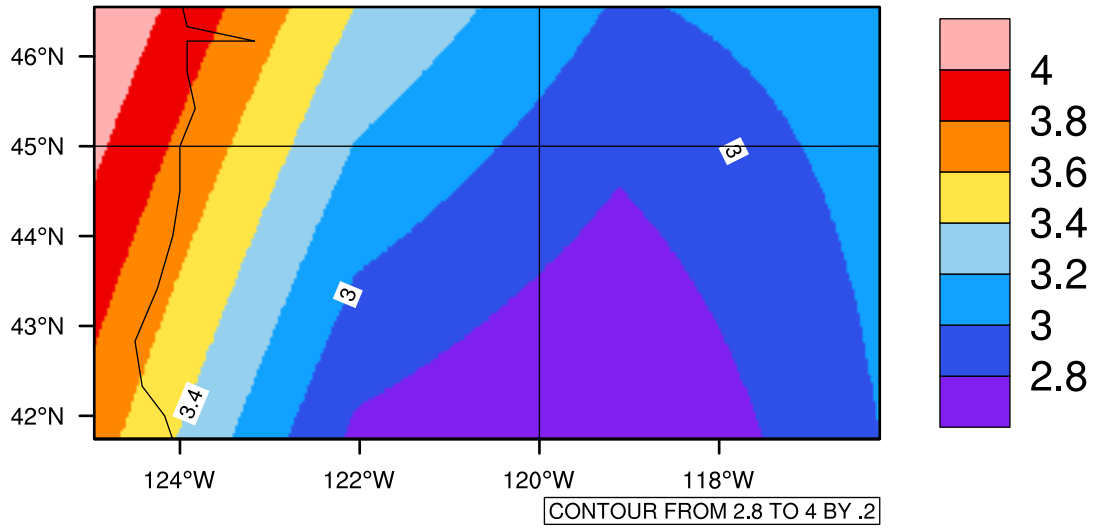
Yearly pr (mm/day) In 2080-2089 GFDL-ESM2M RCP45 - Oregon
